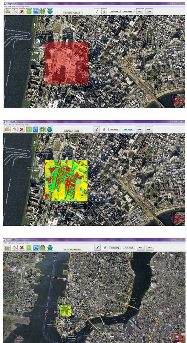
Fig. 2. Different views of the developed tool. Selection of an area to be classified in New York City (top). Unsupervised classification result provided by our implementation of k-means superimposed on the tool (middle). Zoom reduction retaining the classified area (bottom).
