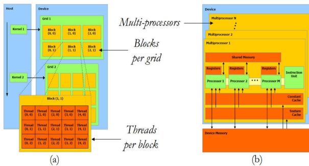
Fig. 3. Schematic overview of a GPU architecture. (a) Threads, blocks and grids. (b) Execution model in the GPU.
